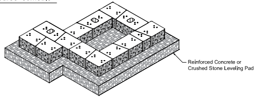
1st Course Isometric
