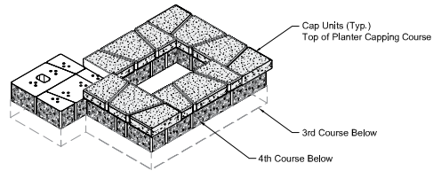
4th Course Capping Isometric
