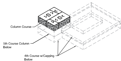
6th Course Isometric
