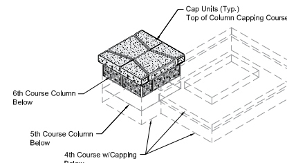
6th Course Capping Isometric
