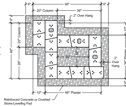
1st Course Plan
