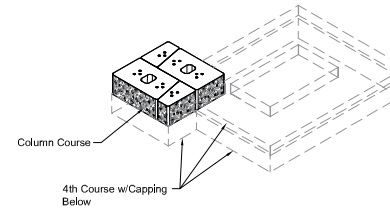
5th Course Isometric
