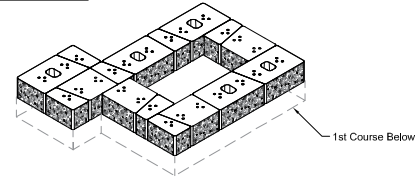
2nd Course Isometric
