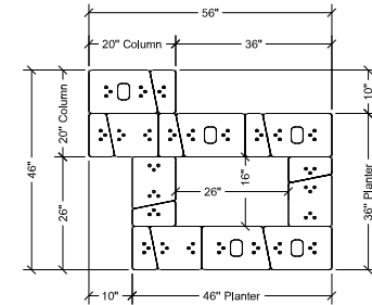
2nd Course Plan
