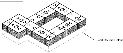
3rd Course Isometric
