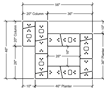
3rd Course Plan
