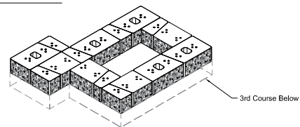
4th Course Isometric
